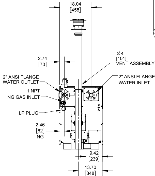
REAR VIEW RSUB-341_A
