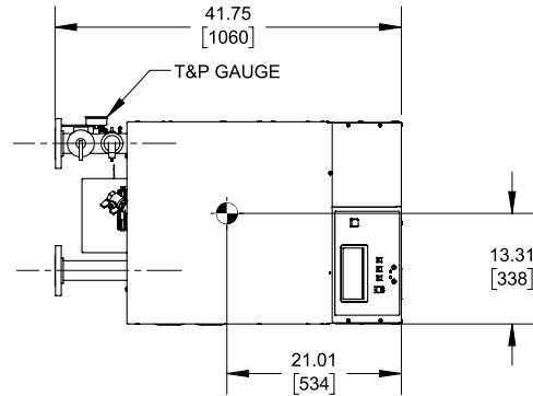
TOP VIEW RSUB-332_A
