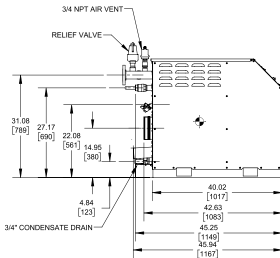
LEFT SIDE VIEW RSUB-333_A
