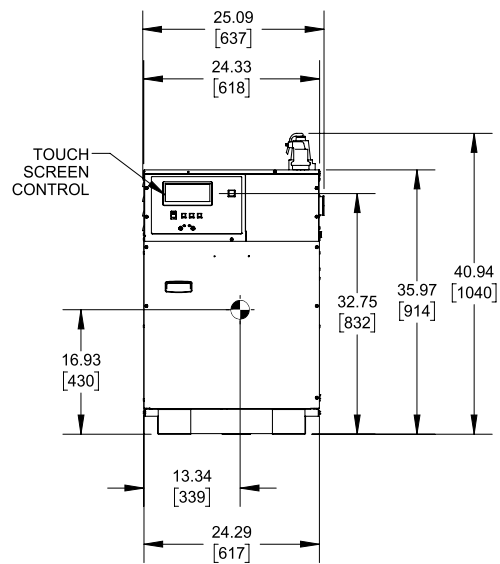
FRONT VIEW RSUB-333_A
