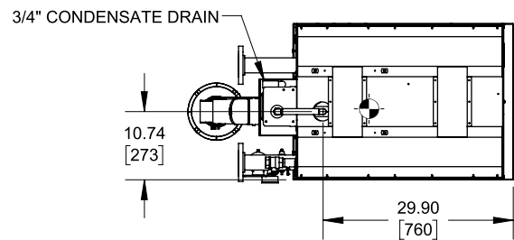
BOTTOM VIEW
