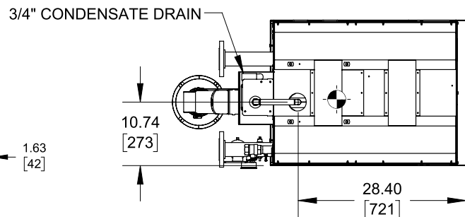
BOTTOM VIEW RSUB-341_A
