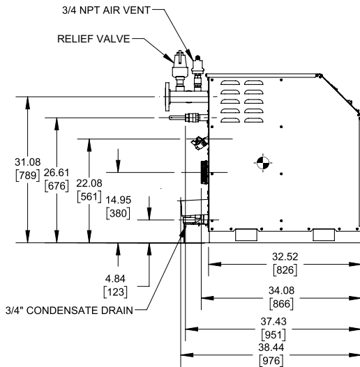
LEFT SIDE VIEW RSUB-332_A
