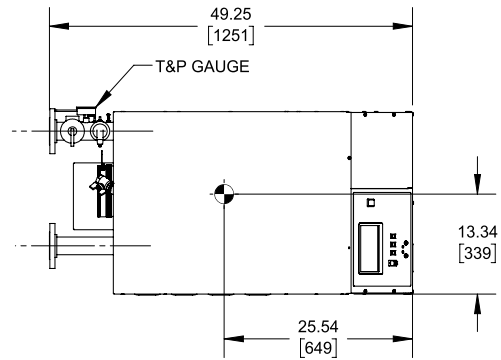
TOP VIEW RSUB-333_A
