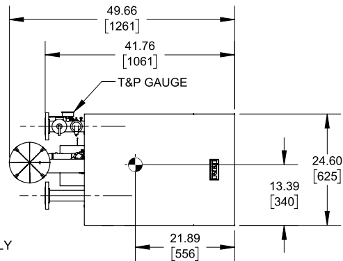
TOP VIEW RSUB-341_A
