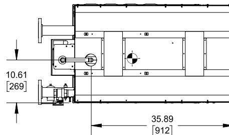
BOTTOM VIEW RSUB-333_A
