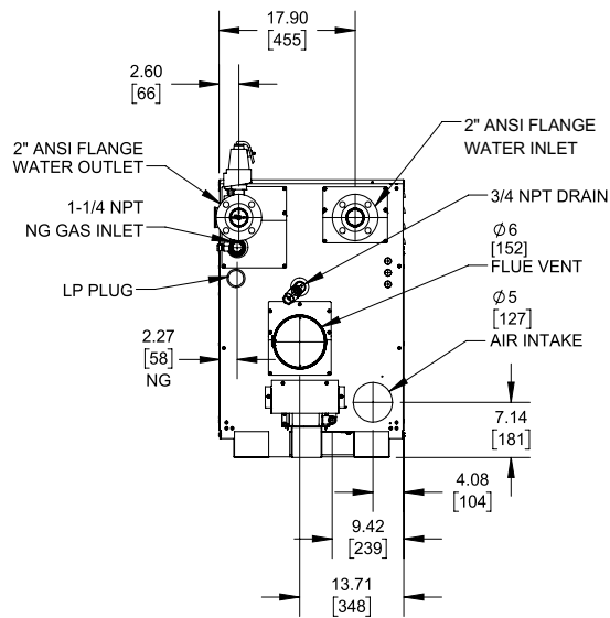
REAR VIEW RSUB-333_A
