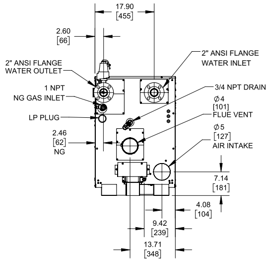
TOP VIEW RSUB-331_A
