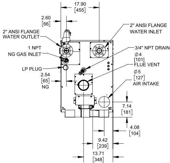
REAR VIEW RSUB-332_A
