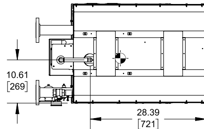
BOTTOM VIEW RSUB-332_A
